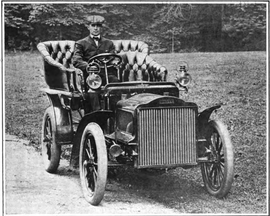
WHITE MODEL E STEAM CAR, FITTED WITH CHANGE SPEED GEAR.
